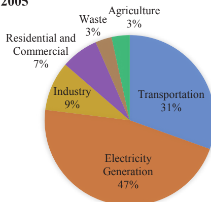
Relative Contributions of Nevada’s Gross GHG Emission by Sector. 2005, 2016, 2025 and 2030
